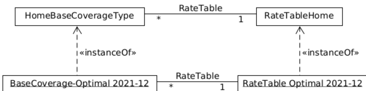
Figure 87. Relationship between Product Components and Tables
