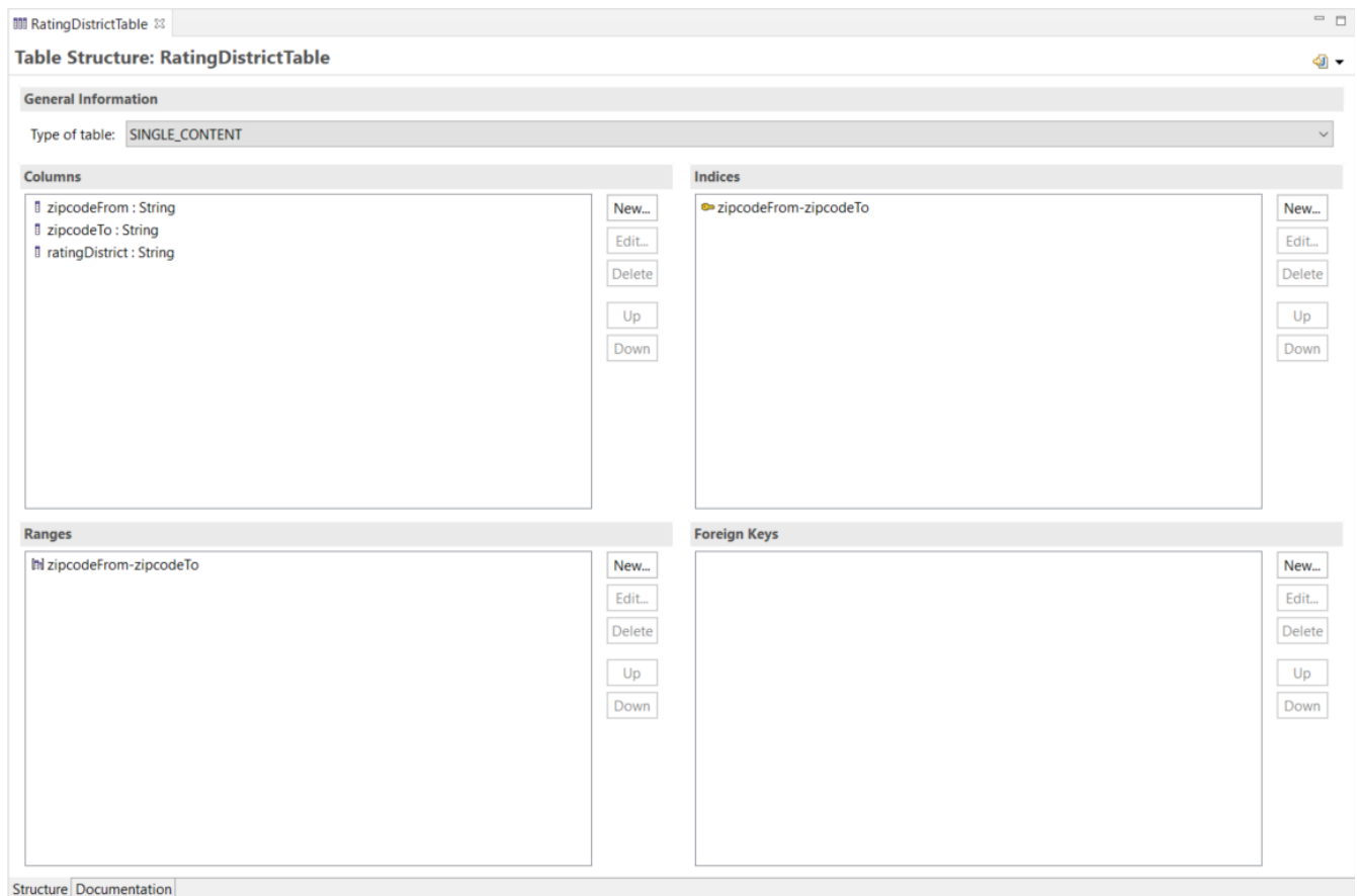
Figure 83. Tablen Structure Rating District Table
