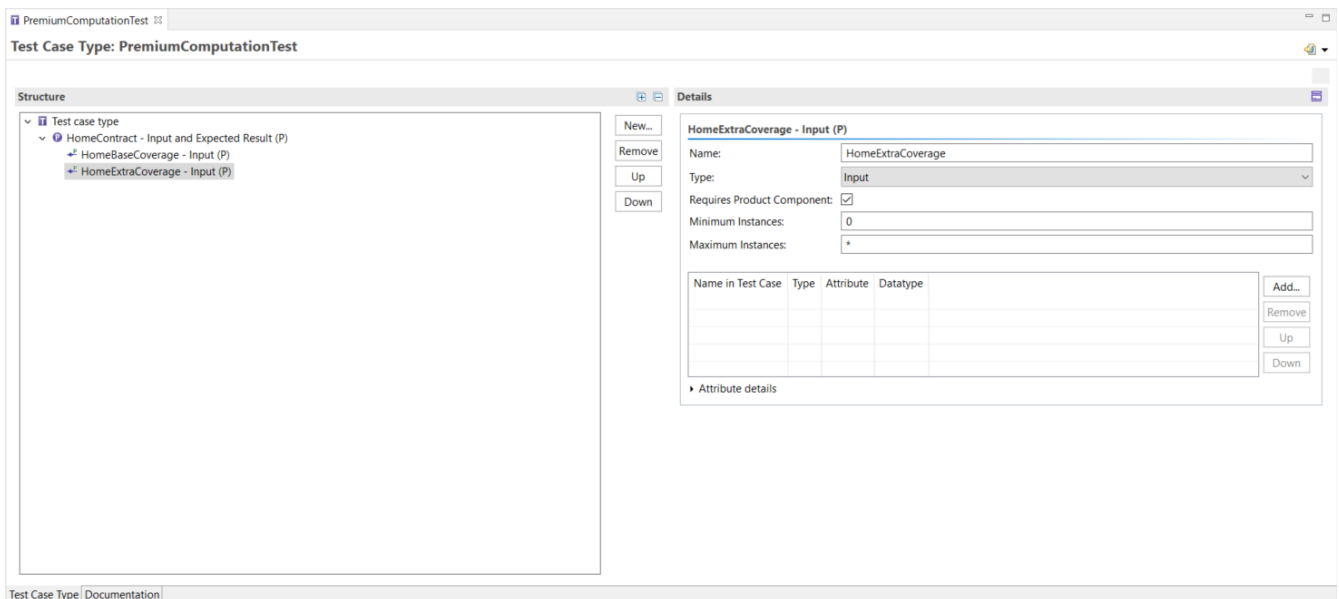
Figure 133. Test Case Type Editor showing the PremiumComputationTest
