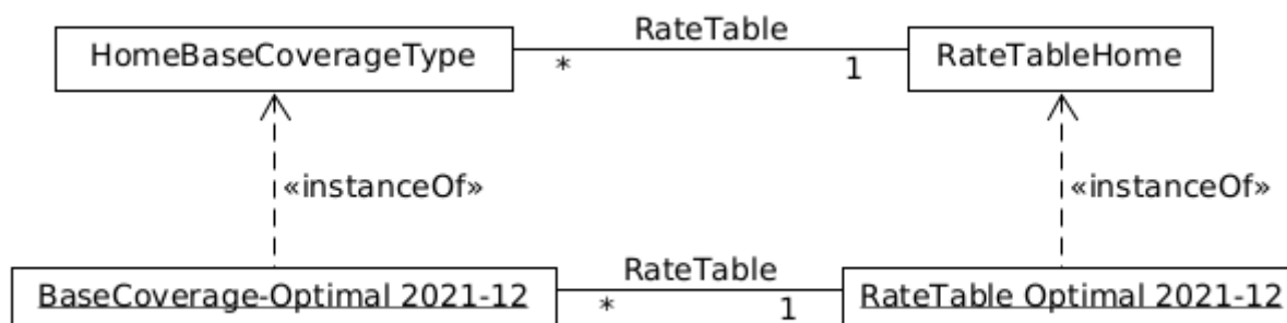
Figure 85. Relationship between Product Components and Tables
