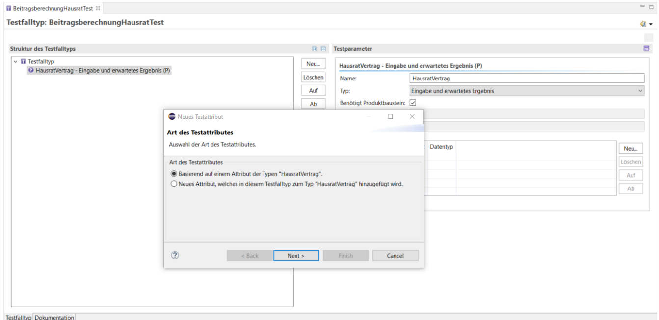
Figure 102. Testattribut anlegen
