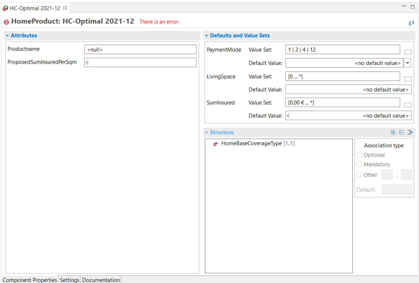
Figure 61. The Product Component Editor for HC-Optimal
