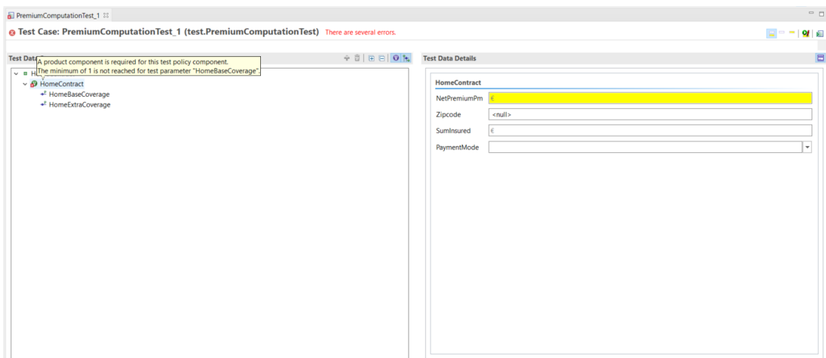
Figure 134. The Test Case Editor hinting at a lacking product component
