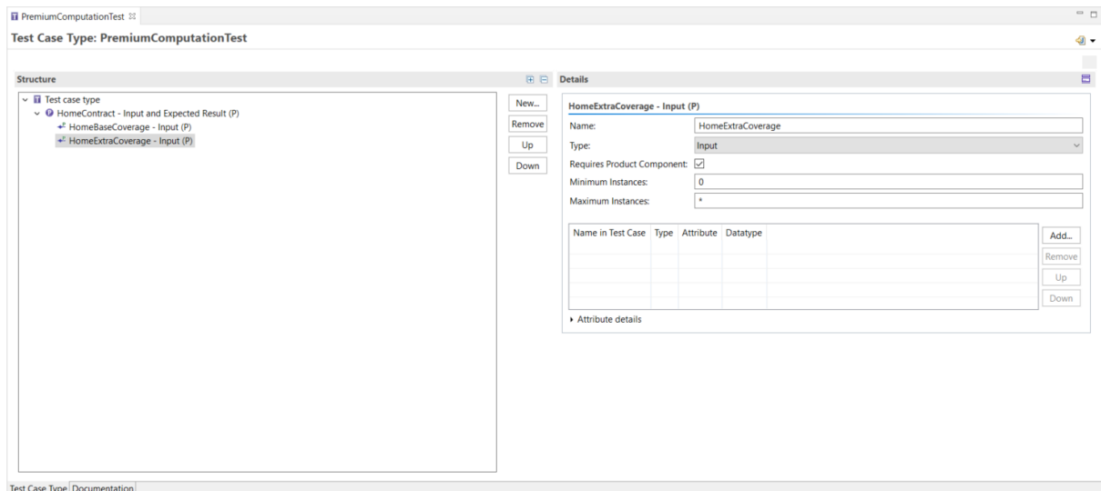
Figure 132. Test Case Type Editor showing the PremiumComputationTest
