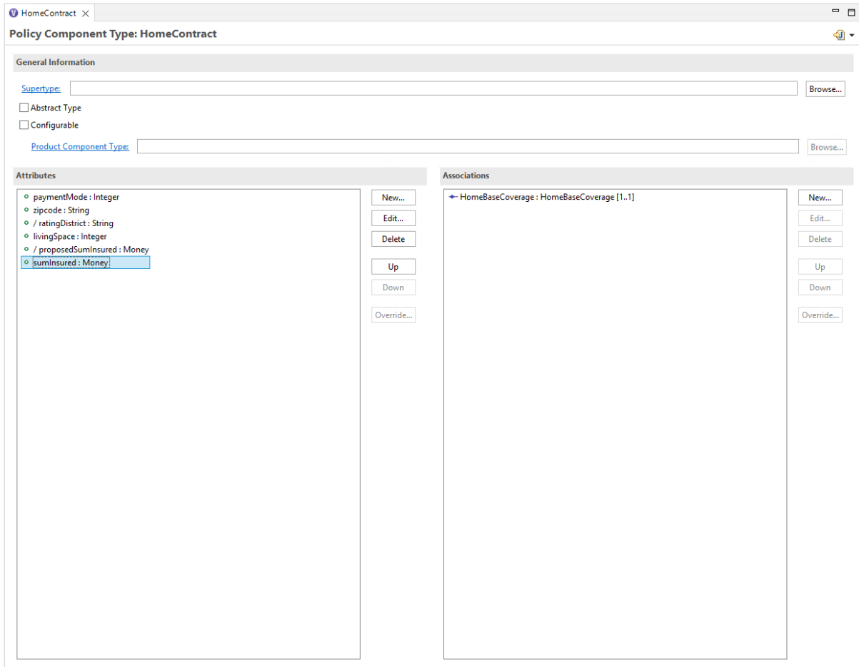
Figure 50. The HomeContract Class
