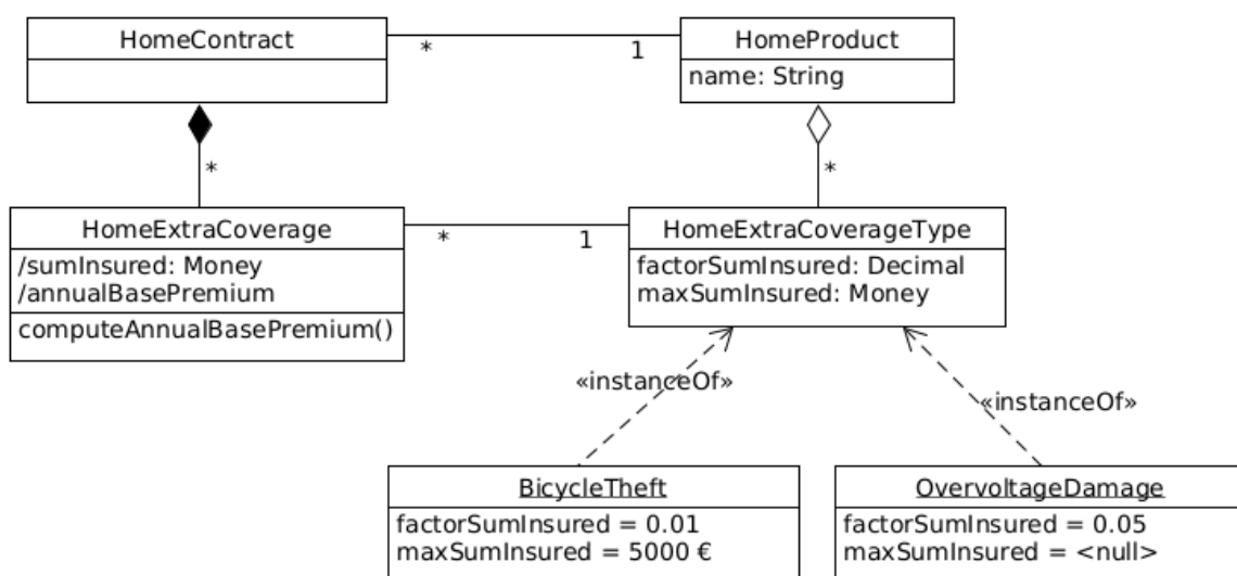
Figure 90. A Section of the Model Showing Extra Coverages with Instances
