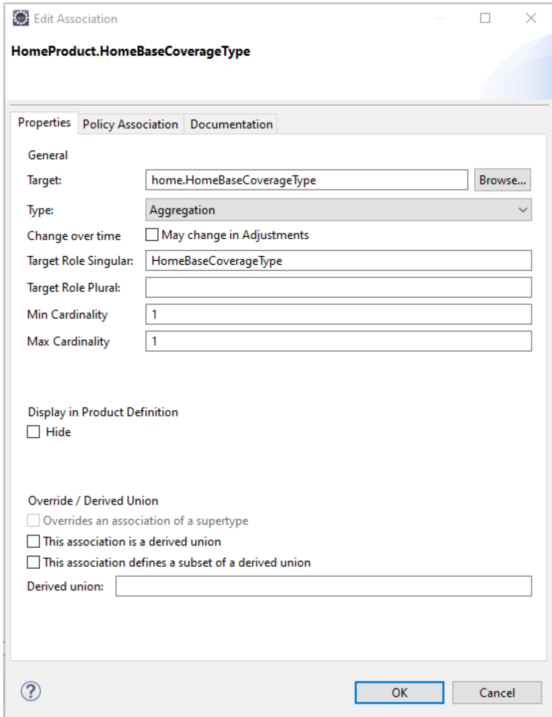
Figure 58. Dialog box for the Relationships between Product Classes
