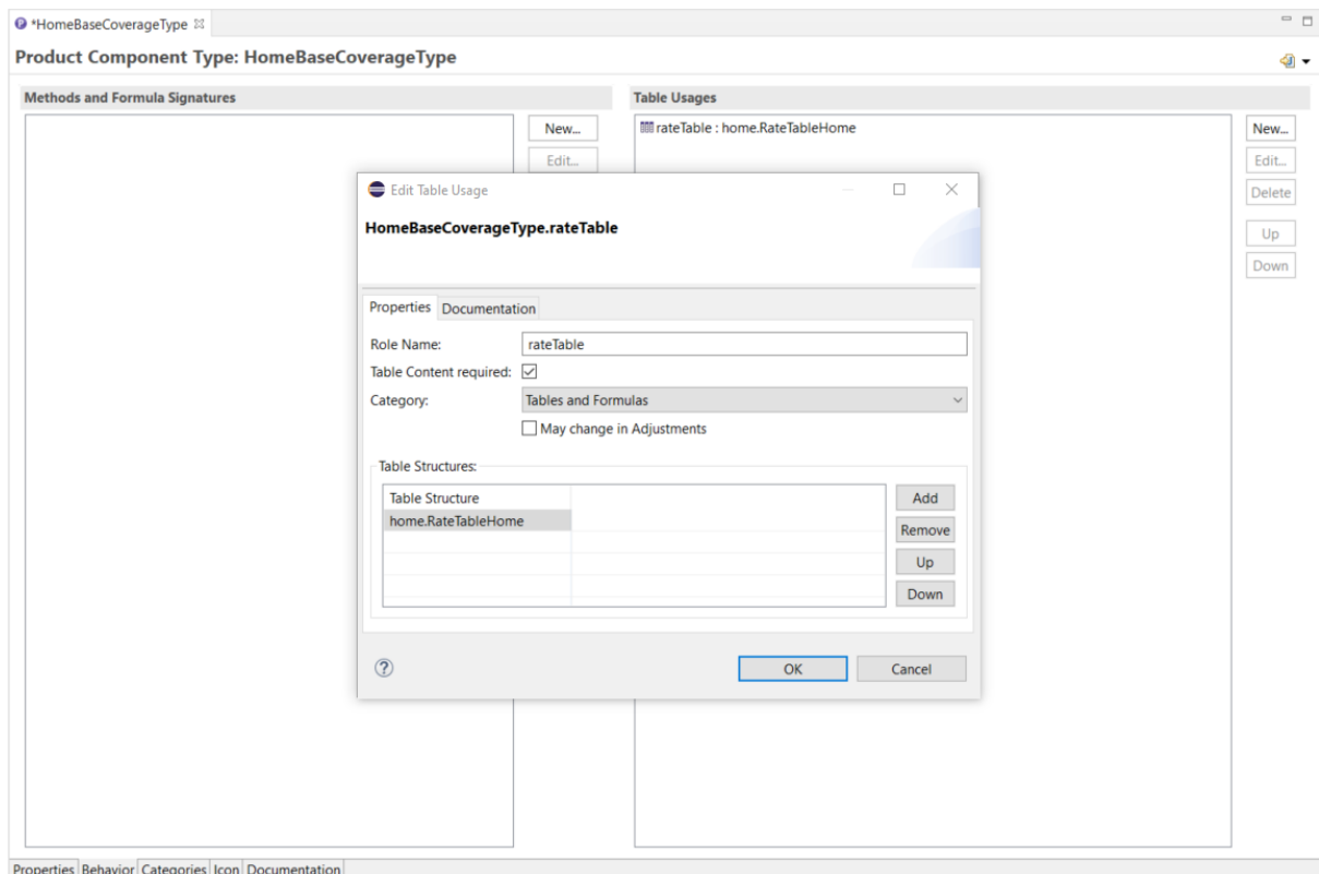
Figure 86. Assigning Table Contents
