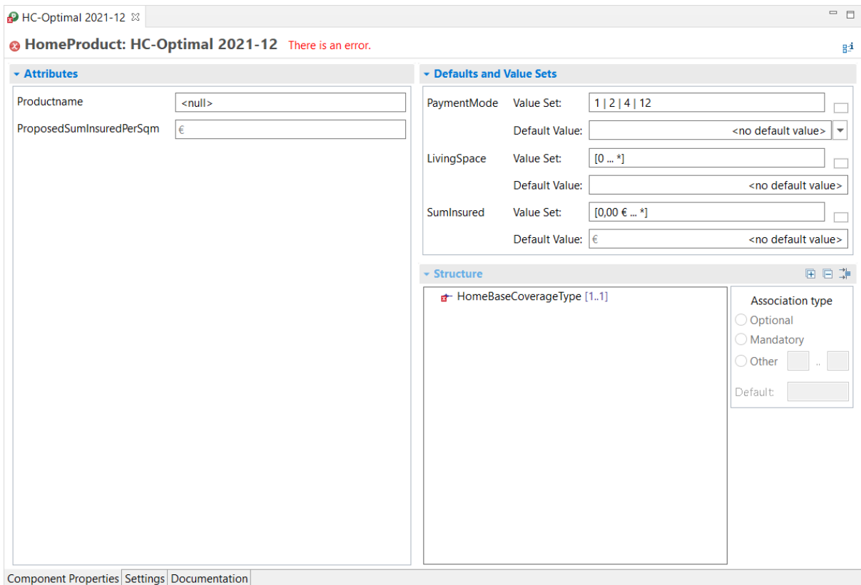
Figure 61. The Product Component Editor for HC-Optimal
