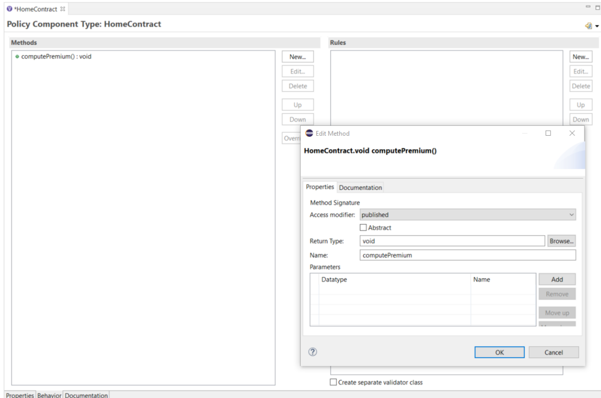
Figure 88. Edit Dialog for Method Signatures
