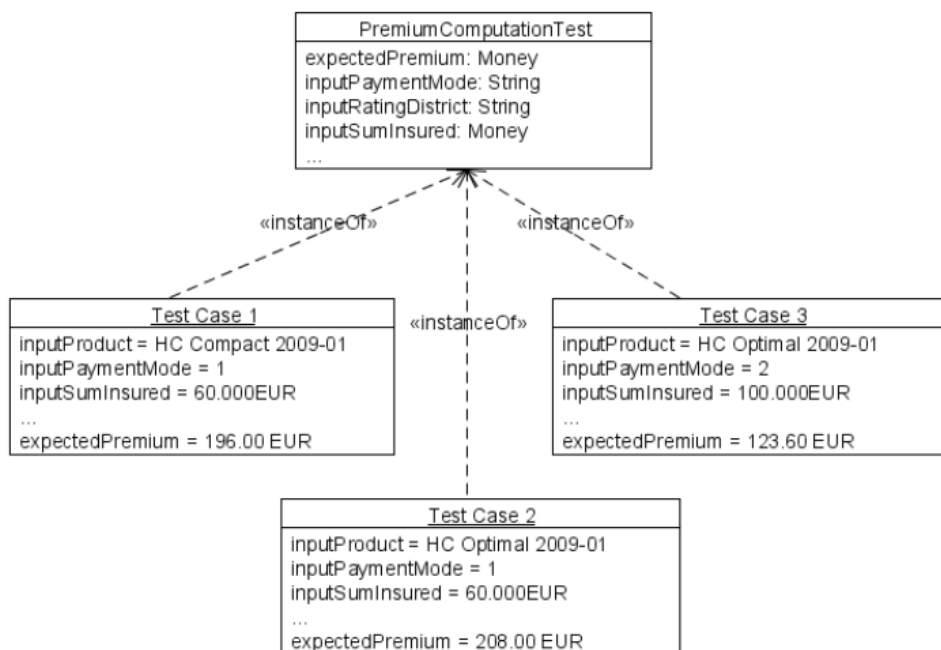
Figure 124. Test cases as instances of the test case type PremiumComputationTest
