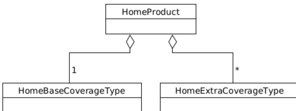
Figure 57. Model of the Product Configuration Classes
